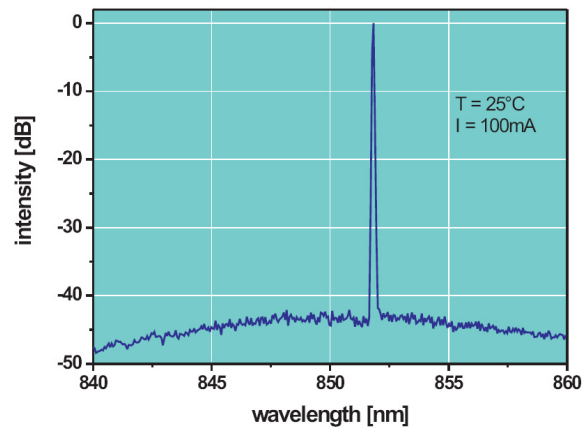
Room Temperature CW Spectrum at 852nm
